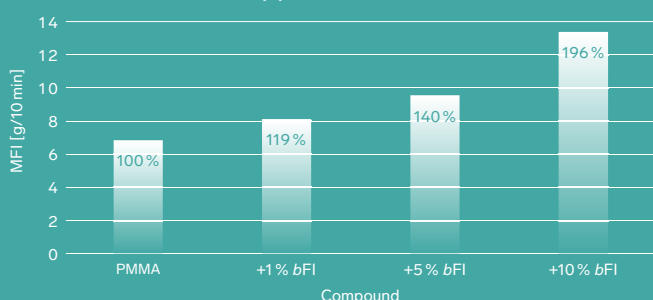
Flow improved properties of bFI applied to PMMA
